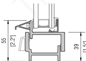
W 4701 - W 4733 | Window
