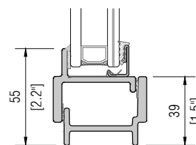
W 4701 - W 4762 | Window
